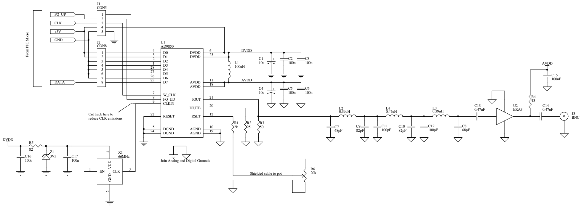
Direct Digital Synthesizer by Steven J. Merrifield, Sept 2003
